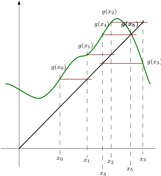
Fixed point iteration
