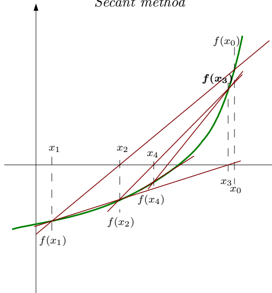
Secant method
