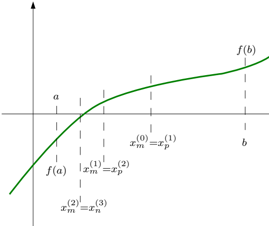
Bisection method
