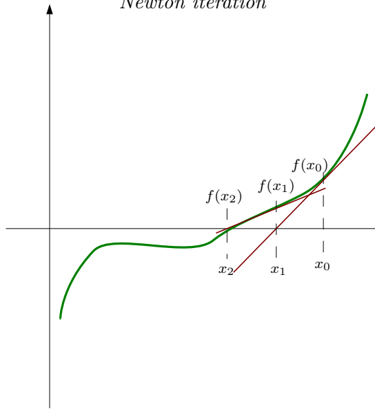
Newton iteration
