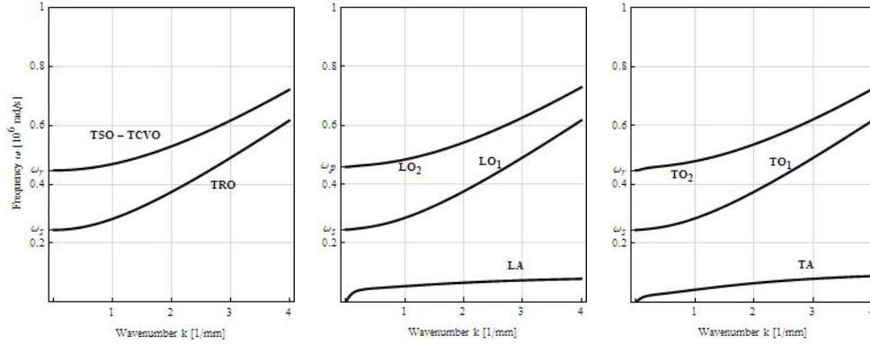
Fig. 5 Dispersion relations \omega = \omega(k) of the relaxed micromorphic model with curvature \|\text{Div}P\|^2 + \|\text{Curl}P\|^2 for the uncoupled (left), longitudinal (center) and transverse (right) waves with non-vanishing gradient micro-inertia. One band-gap is possible.
